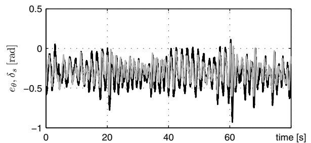
Fig. 10. Ex. B—Orientation tracking error e_\theta (■), skid-slip angle \delta_s (■).
