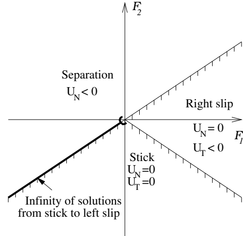
Fig. 3. Case \mathcal{F} = \frac{\lambda+3\mu}{\lambda+\mu} = 3 - 4\nu . Problem (27) admits either a unique or an infinity of solutions.
