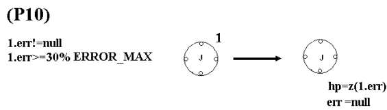
Fig. 17. cp-graph grammar production for virtual hp .
