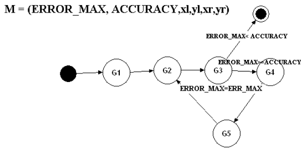
Fig. 5. Control diagram for a cp-graph grammar system modeling the hp -FEM.
