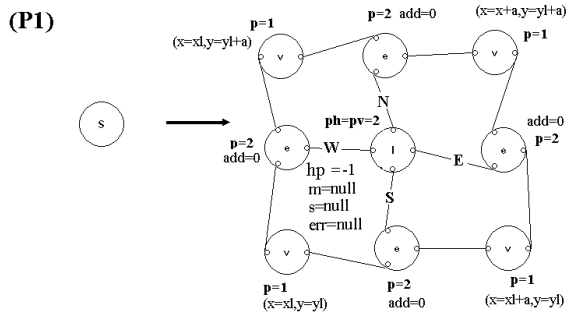
Fig. 6. One of the cp-graph grammar productions for generation of the initial mesh.
