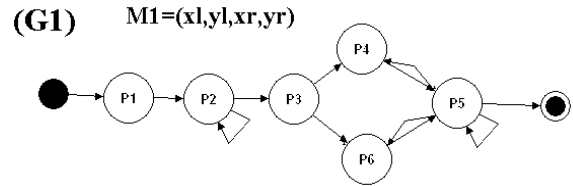
Fig. 12. Control diagram for the graph grammar G1 for generation of the initial mesh.
