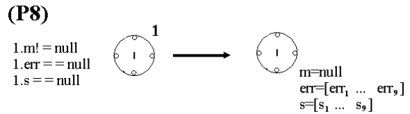
Fig. 14. cp-graph grammar production for calculating the vectors of the solution and error on the basis of a matrix.
