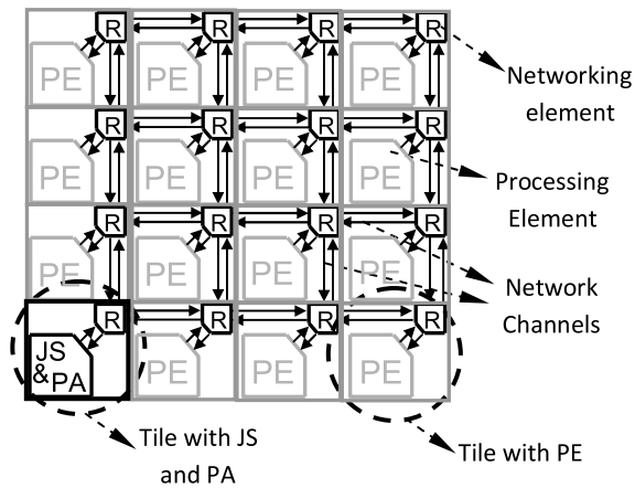
Fig. 1. Tiled CMP ( 4 \times 4 2D-mesh) with an integrated job scheduler and processor allocator.
