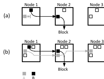
Fig. 3. Packet A is blocked behind B—wormhole flow control (a), packet A can pass packet B—virtual channel flow control (b).
