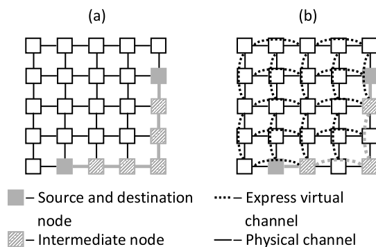
Fig. 4. Regular structure and example of transmission (a), the same transmission in a structure with express virtual channels (b).
