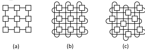
Fig. 2. 2D-mesh and 2D-torus networks: 3-ary 2-mesh (a), 3-ary 2-cube (b), folded 3-ary 2-cube (c).
