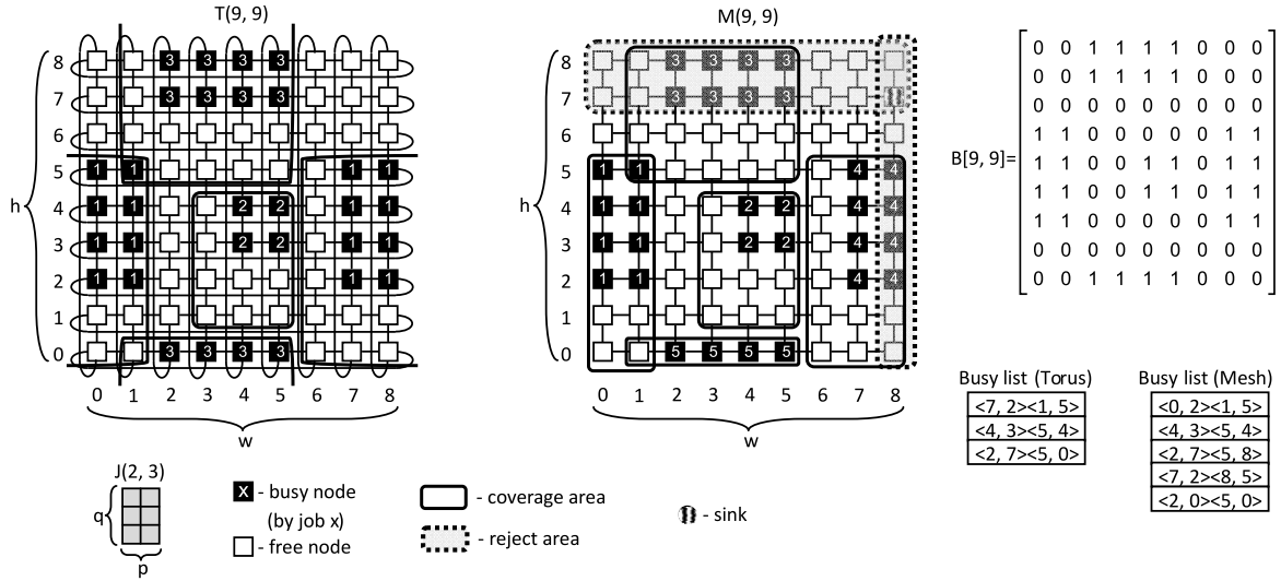
Fig. 5. Torus T(9,9) and mesh M(9,9) , busy and free nodes, coverage areas, busy array, busy lists.
