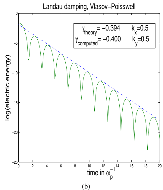
Fig. 1. Evolution of the logarithm of the electric energy in the case of the Landau damping: (a) Vlasov-Darwin, (b) Vlasov-Poiswell.
