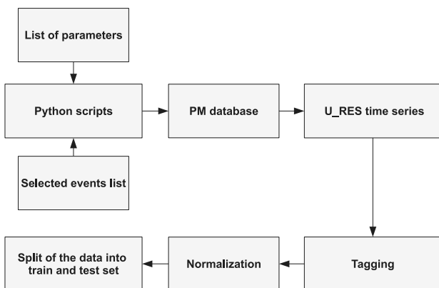
Fig. 5. Procedure for the extraction of voltage time series with selected events from the PM database using U_{RES} as an example.
