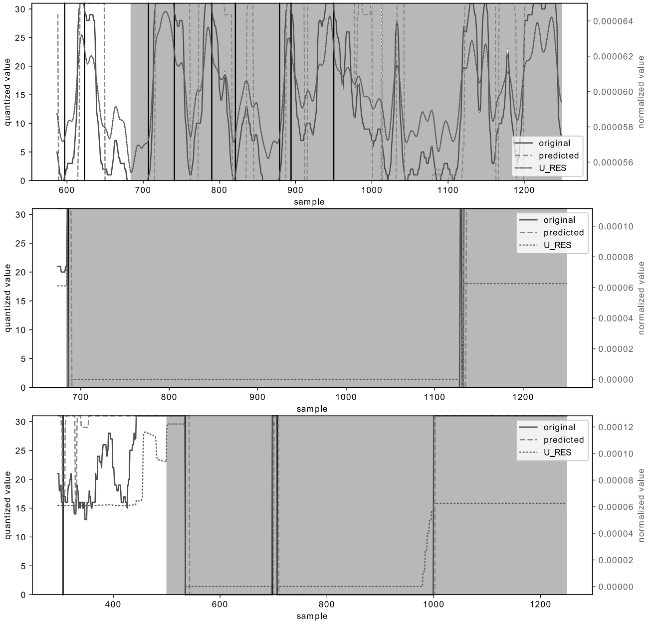
Fig. 8. Visualization of the proposed anomaly detector results for three example series using the LSTM model with two layers (64 and 32 cells), look_back = 256 and grid = 32. The gray span indicates the area labelled in data as an anomaly (from QUENCHTIME until the end of a series); the thick vertical black lines are the point detector marked as a start of anomaly (trigger points); the dotted grey line (and scale on the right) represents the original, normalized signal before quantization, while the solid and dashed lines represent the real and the predicted quantized signal, respectively.
