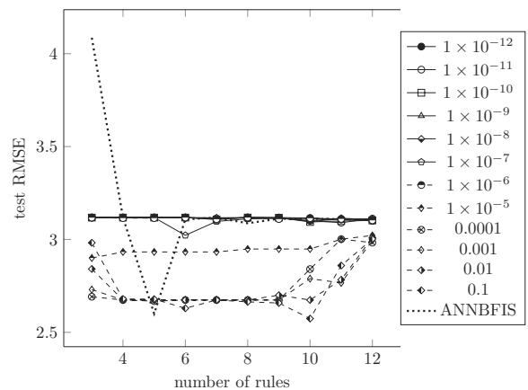
Fig. 15. Root mean square errors for the ‘synthetic’ data set with the FCOM-ANNBFIS neuro-fuzzy system.
