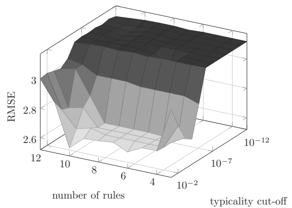
Fig. 15. Root mean square errors for the ‘synthetic’ data set with the FCOM-ANNBFIS neuro-fuzzy system.
