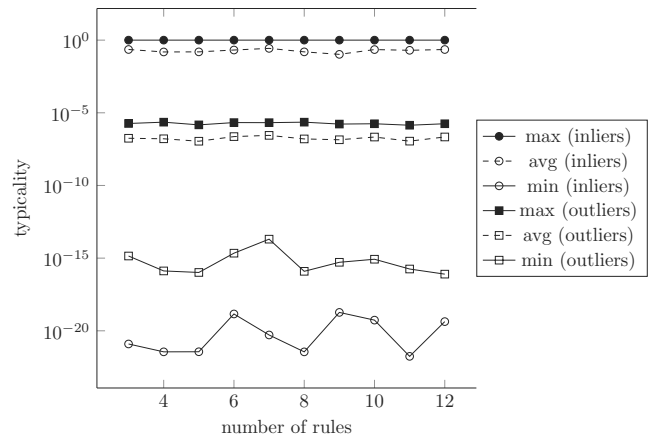
Fig. 8. Extreme and average values of typicalities of informative objects (inliers) and non-informative items (outliers) in the 'blood' data set produced by the ANNBFI neuro-fuzzy system with the FCOM clustering algorithm.
