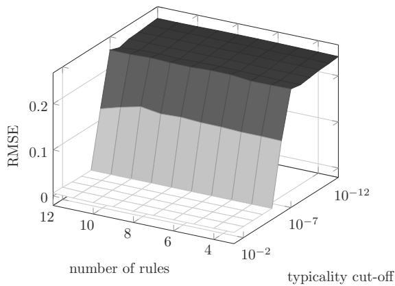
Fig. 10. Root mean square errors for the ‘carbon’ data set with the FCOM-TSK neuro-fuzzy system.
