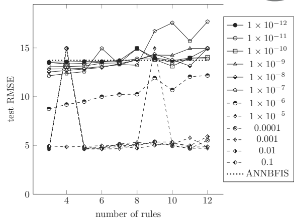
Fig. 19. Root mean square errors for the ‘power’ data set with the FCOM-ANNBFIS neuro-fuzzy system.
