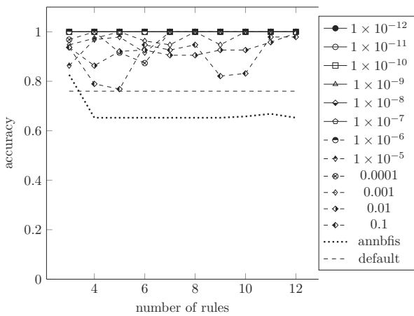
Fig. 5. Classification accuracy of the 'parkinsons' data set with the ANNBFI system with FCOM and various typicality cut-offs ('annbfis' stands for the reference ANNBFI system with the FCM clustering algorithm, 'default' for the majority class frequency in the data set).
