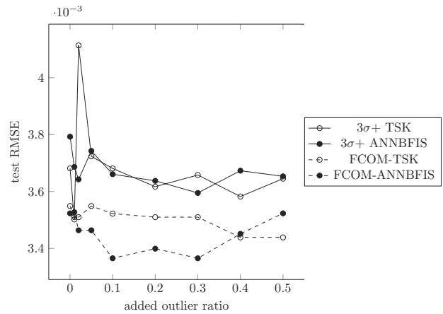
Fig. 31. Comparison of the proposed approach with the 3\sigma pre-processing technique for various ratios of outliers in the ‘carbon’ data set.
