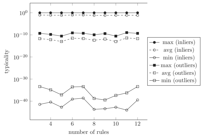
Fig. 7. Extreme and average values of typicalities of informative objects (inliers) and non-informative items (outliers) in the 'htru' dataset produced by the ANNBFI neuro-fuzzy system with the FCOM clustering algorithm.
