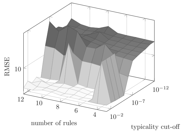
Fig. 20. Root mean square errors for the ‘power’ data set with the FCOM-ANNBFIS neuro-fuzzy system.
