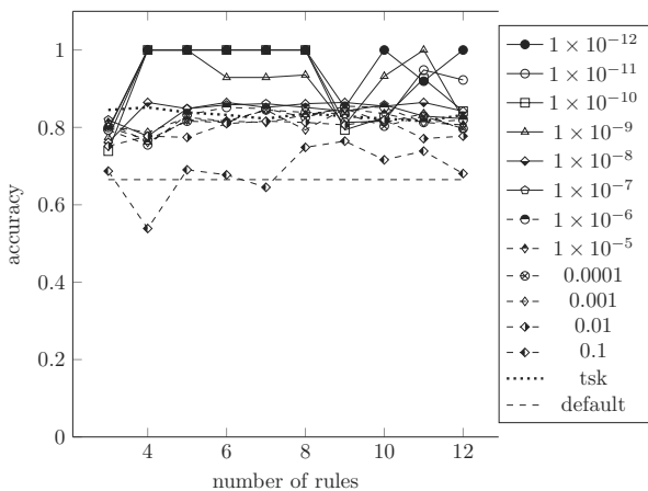
Fig. 6. Classification accuracy of the 'vertebral' data set with the TSK system with FCOM and various typicality cut-offs ('tsk' stands for the reference TSK system with the FCM clustering algorithm, 'default' for the majority class frequency in the data set).
