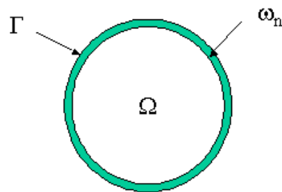
Fig. 5. Sequence of neighbourhoods \omega_n of \Gamma .
