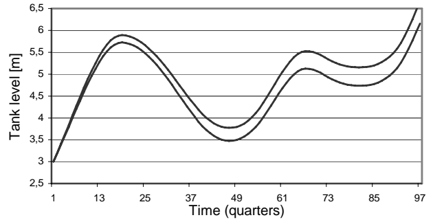
Fig. 7. Estimated bounds on the tank level; L = 0 .
