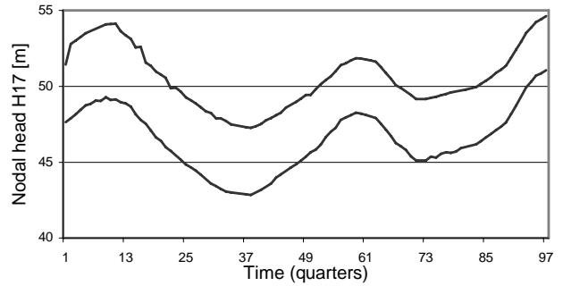
Fig. 9. Estimated bounds on the nodal head H17; L = 0 .
